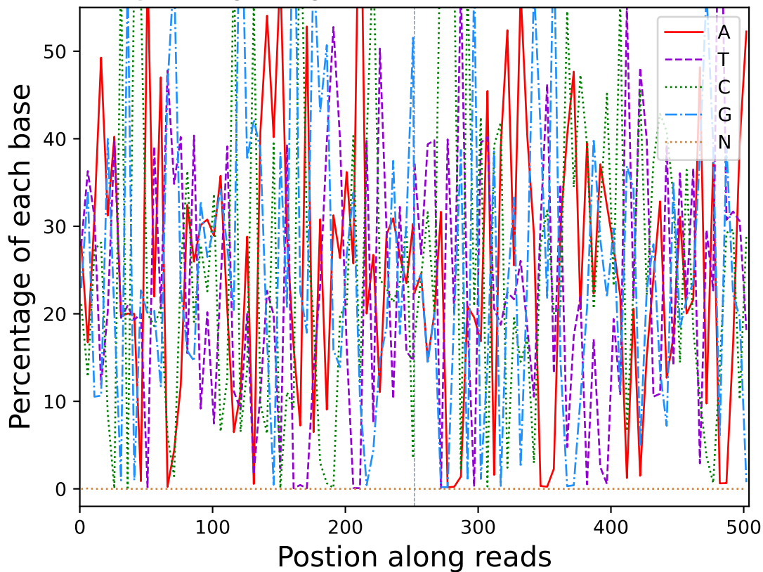
Base percentage along reads (R20208)
